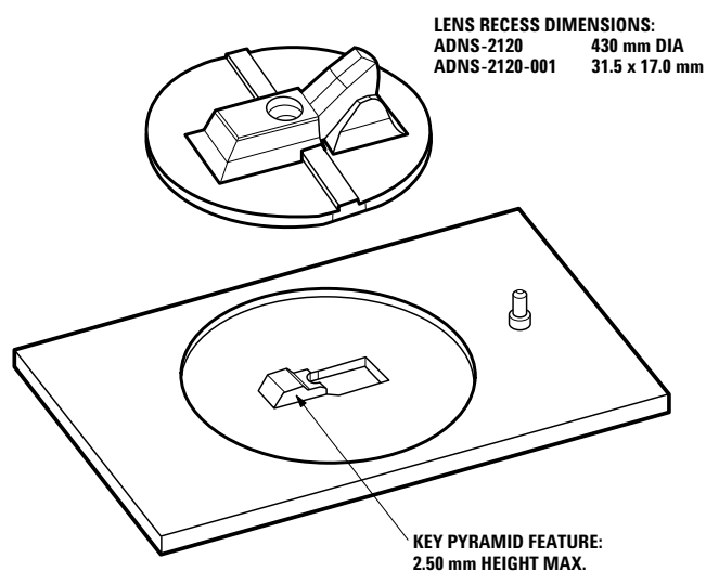
Figure 3. Illustration of base plate mounting features.
